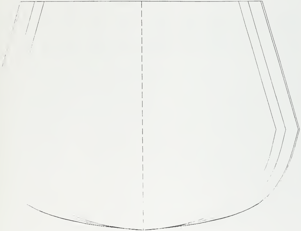
COMP_CB.C Body Plan (1 component) Scale = 1:100
